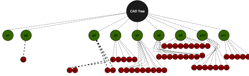
Fig. 8. CAD tree of unchanged cells from F_1 incremented by f_4 .
