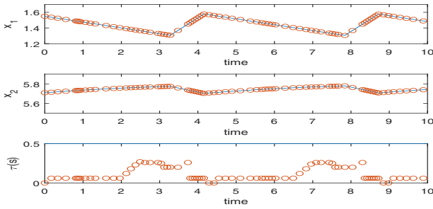
Fig. 4. Trajectory of the closed-loop switched system with the safety controller designed for the symbolic model starting at the initial state x = [1.55, 5.71]^T ; The sampling instants generated while computing the symbolic abstraction.
