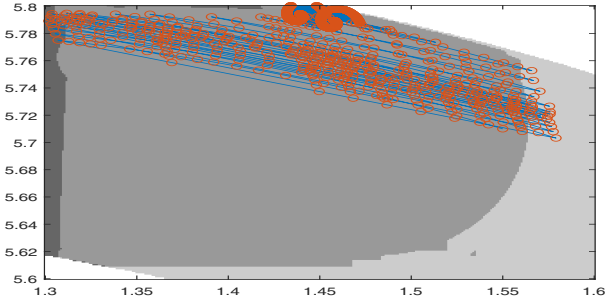
Fig. 3. Safety controller for the symbolic model (dark gray: mode 1, light gray: mode 2, medium gray: both modes are active, white: uncontrollable states) and the trajectory of the closed-loop switched system.
