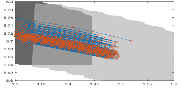
Fig. 1. Safety controller for the symbolic model(dark gray: mode 1, light gray: mode 2, medium gray: both modes are active, white: uncontrollable states) and the trajectory of the closed-loop switched system.
