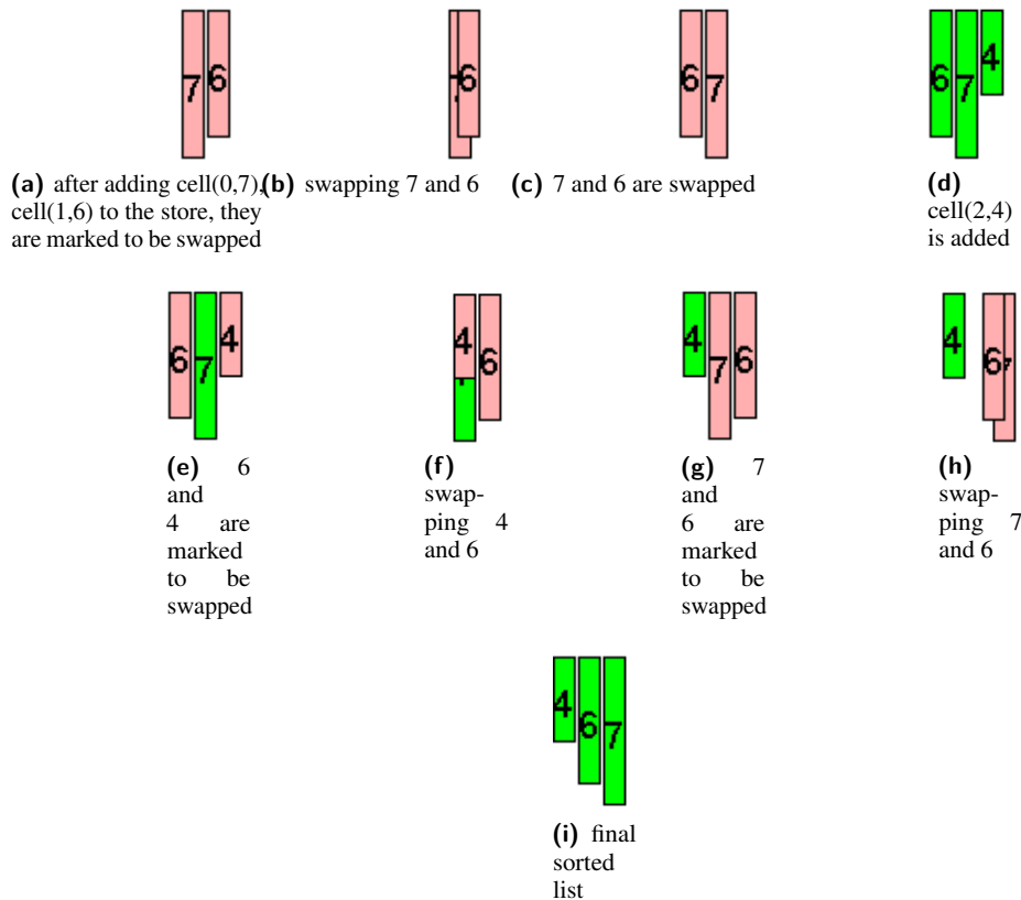
■ Figure 4 Sorting an array of numbers through a rule annotation.
