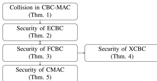
Fig. 1. Proof sketch
