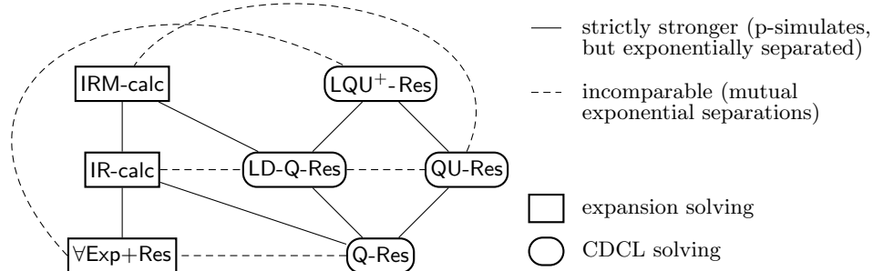
Fig. 1. QBF resolution calculi [7] and their simulation order.
