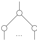
Figure 2: Family of string diagrams
