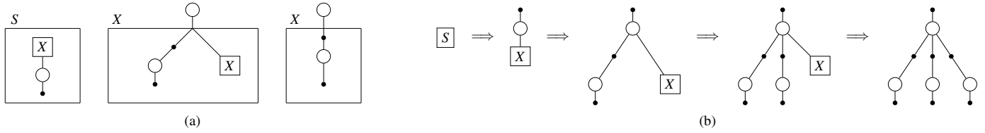
Figure 3: A B-edNCE grammar (a) and a concrete derivation from it (b).
