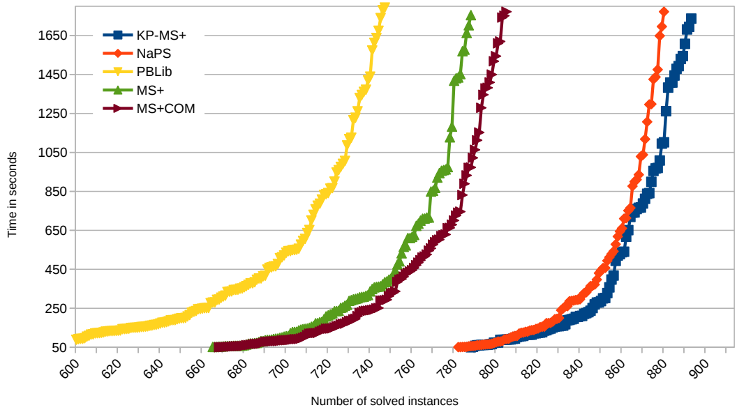
Figure 5: Cactus plot for OPT-BIGINT-LIN division.
