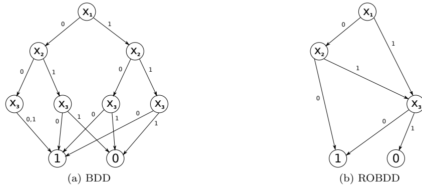
Figure 3: Construction of a BDD (left) and a ROBDD (right) for 2x_1 + 3x_2 + 5x_3 \leq 6 .
